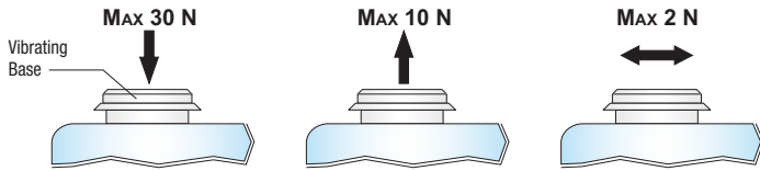
Fig. 2: maximum load limits for vibrating base
