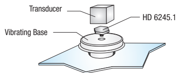
Fig. 3: Adhesive Mounting
